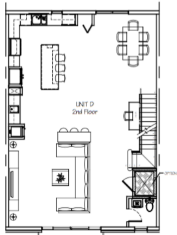
2 UNIT D SECOND FLOOR PLAN SCALE: 1/4" = 1'-0"
