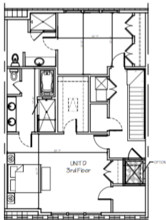
3 UNIT D THIRD FLOOR PLAN SCALE: 1/4" = 1'-0"
