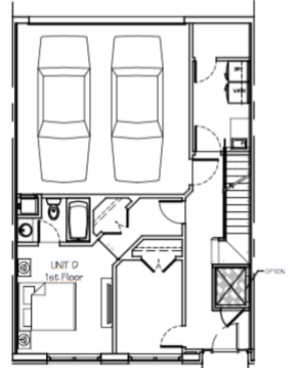
1 UNIT D FIRST FLOOR PLAN SCALE: 1/4" = 1'-0"
